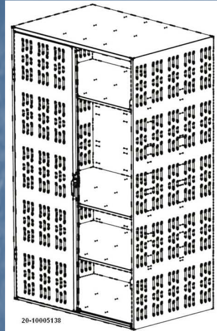
Tool/Spare Parts Storage Cabinet, Dimensions; 1200 mm W x 2000 mm H x 800 mm D
