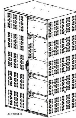
Tool/Spare Parts Storage Cabinet, Dimensions; 1200 mm W x 2000 mm H x 800 mm D
